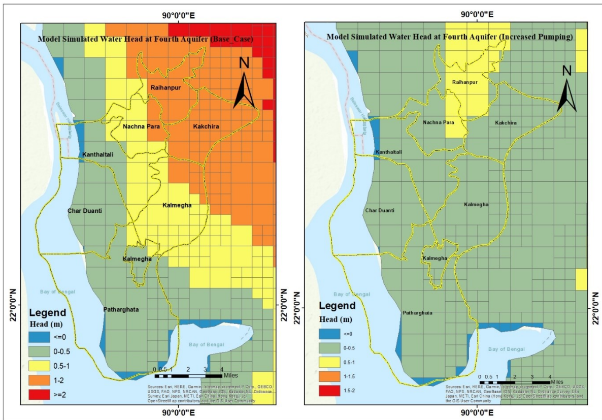
Figure 17: comparison between deep aquifer in Base Case condition in December 2019 (left) and in increased pumping condition in December 2025 (right)
