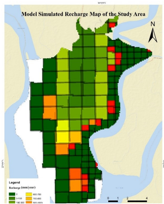
Figure 38: the model simulated actual recharge in Patharghat Upazila in 2019
