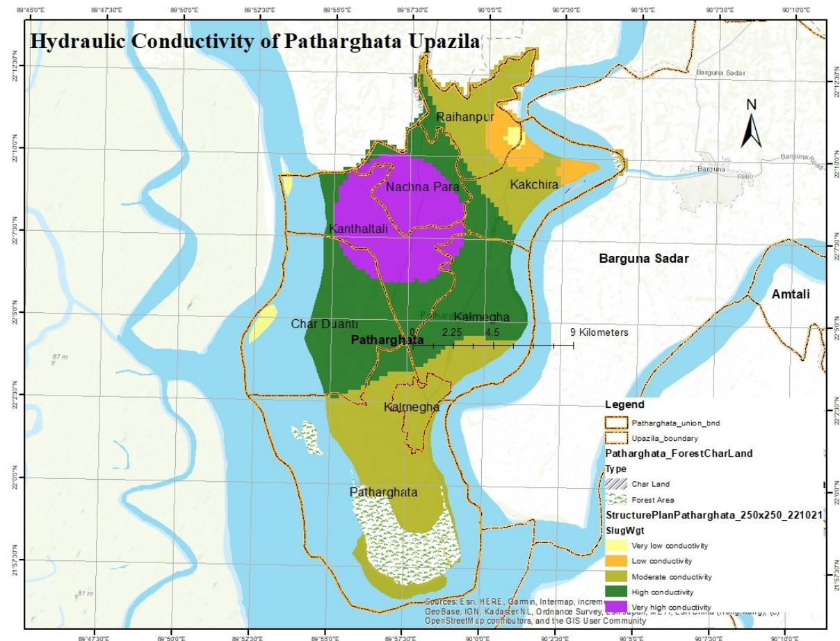
Figure 36: Hydraulic conductivity of Patharghata Upazila from Slug test
