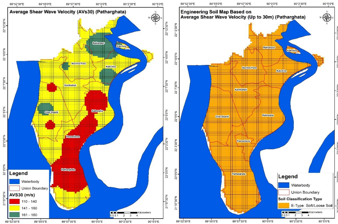
Figure 43: Average share wave velocity map
