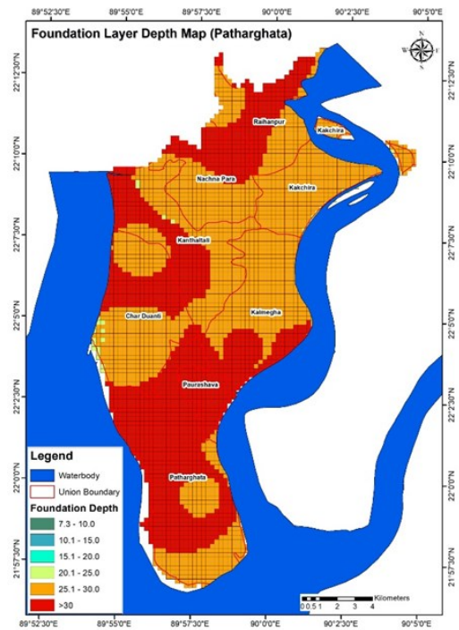
Figure 41: Foundation layer depth map
