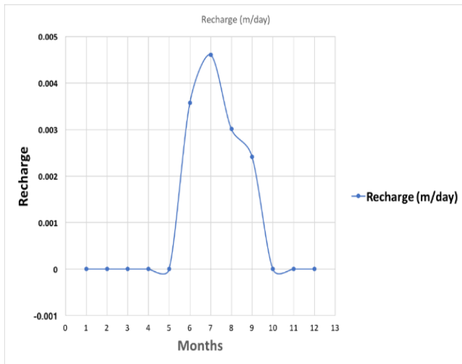
Figure 39 : potential recharge measured by Chaturvedi (1973) formula
