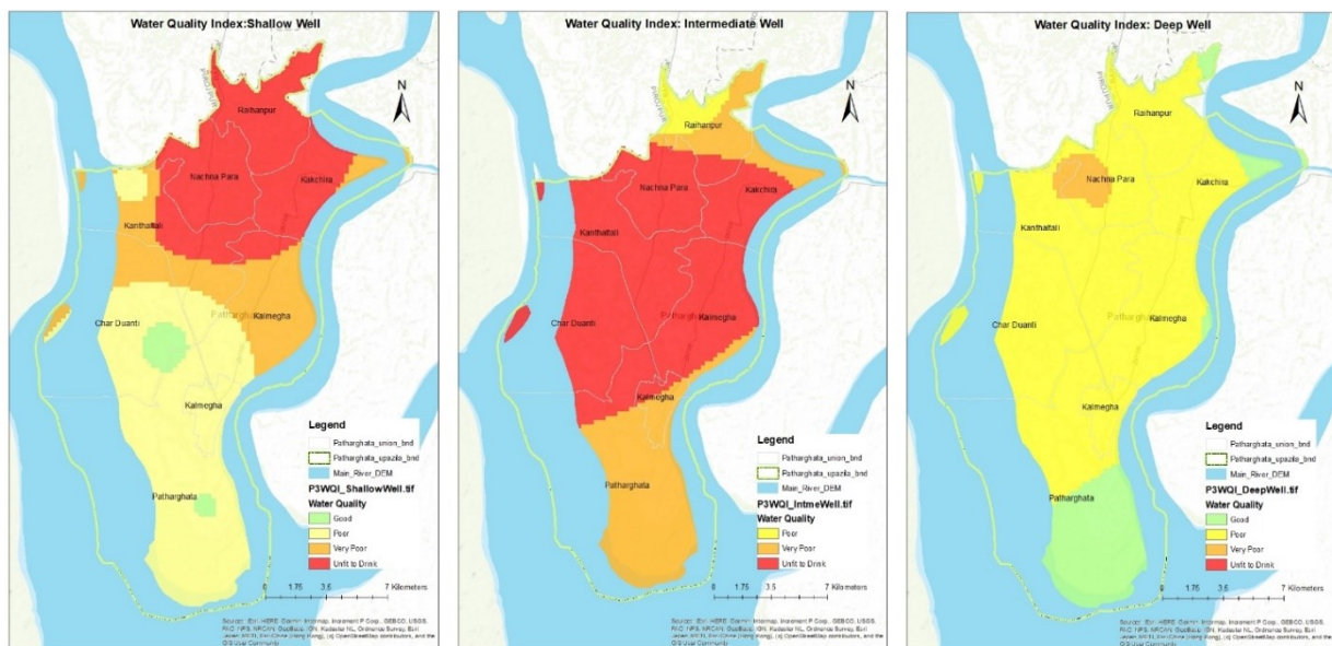
Figure 35: WQI of shallow, intermediate and deep aquifer
