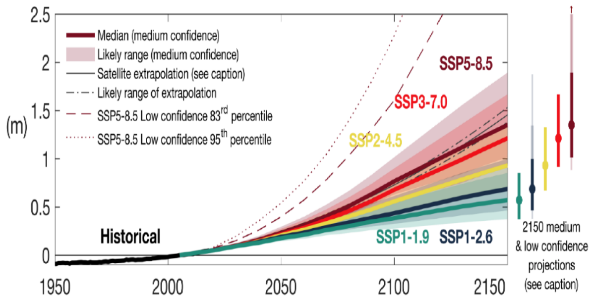
Figure 22 Projected global mean sea level rise (m) under different SSP-RCP scenarios based on CMIP6 models
