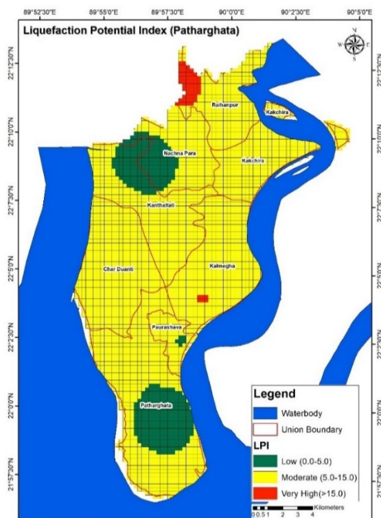
Figure 44: Liquefaction Potential Index map of Study Area
