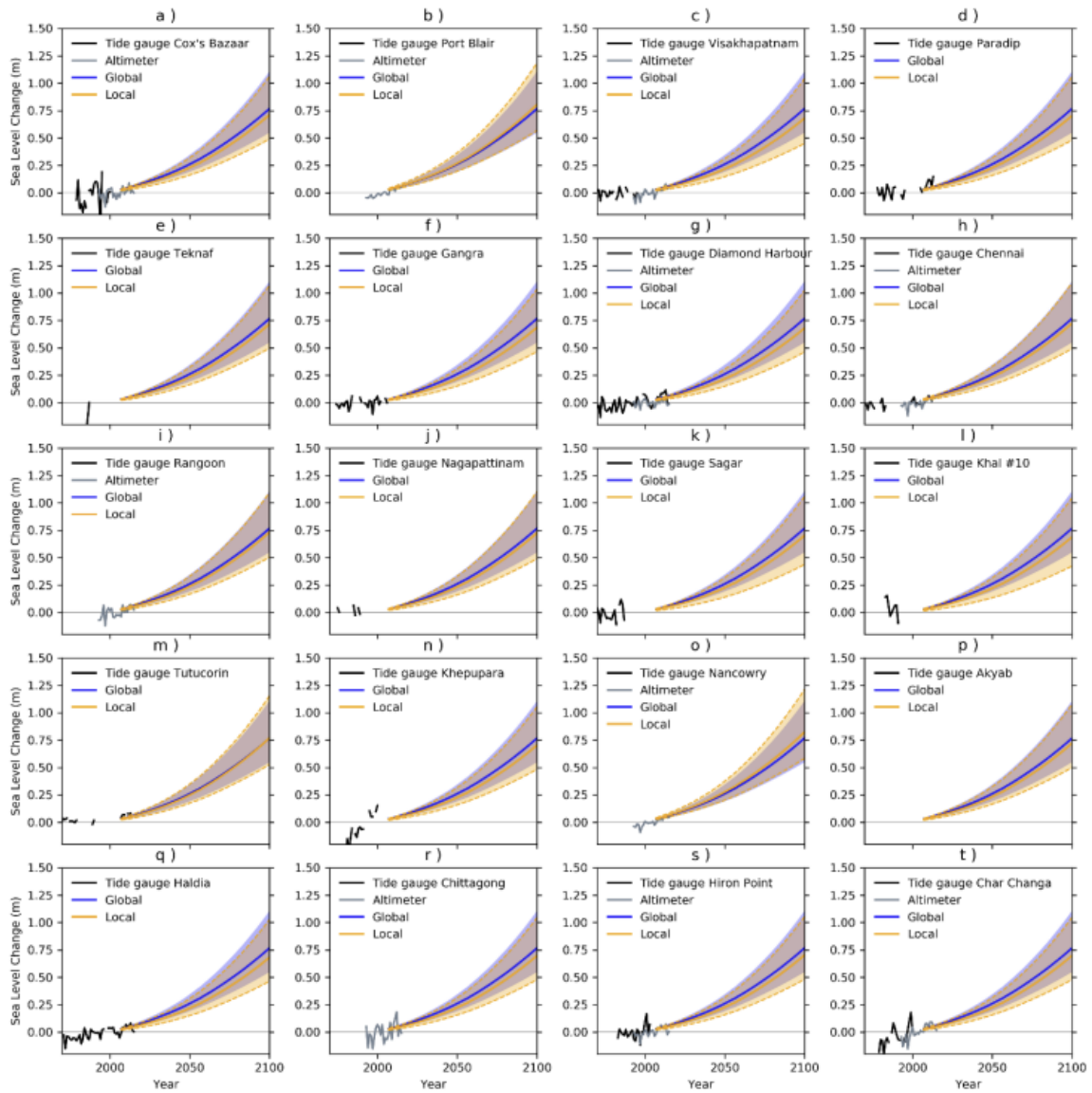
Figure 23 21st-century sea-level projections for RCP8.5
