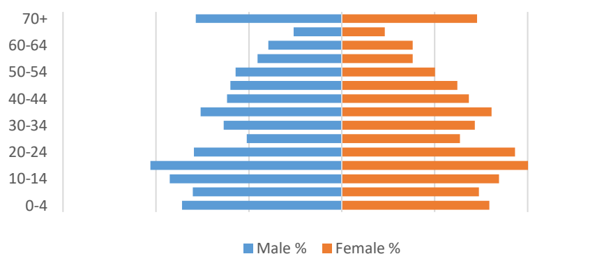
Age Sex Pyramid of Patharghata Upazila(2021)
