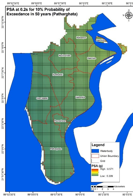
Figure 7: Probabilistic Seismic Hazard Assessment (PSHA): PGA and PSA
